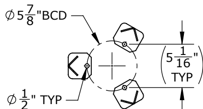
SECTION U-U
